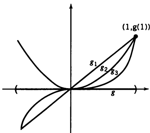
Figure 8.1.2 g_n(x) = x^n .
