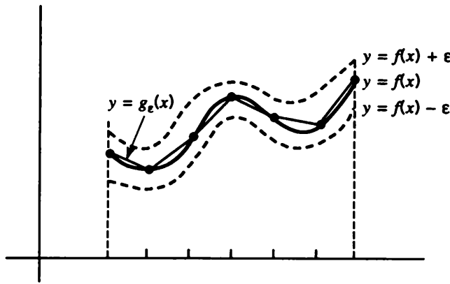
Figure 5.4.5 Approximation by piecewise linear function.
