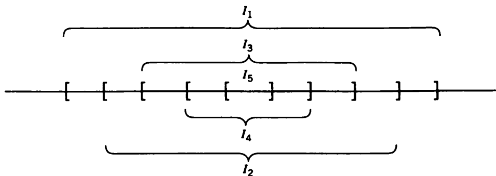
Figure 2.5.1 Nested intervals
