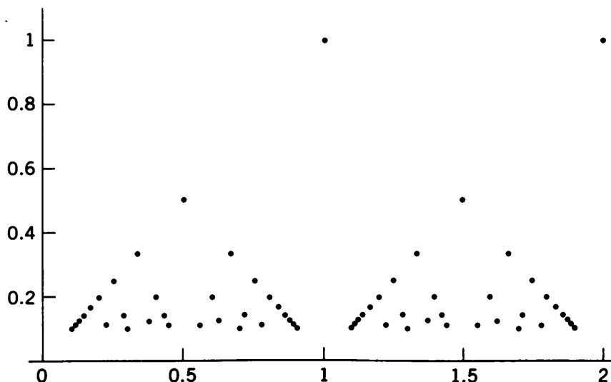
Figure 5.1.2 Thomae's function.
