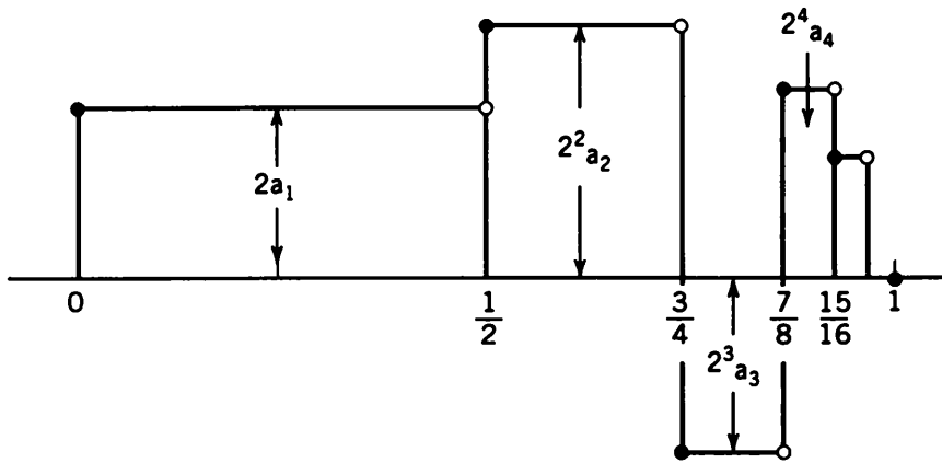
Figure 10.2.1 The graph of \varphi .
