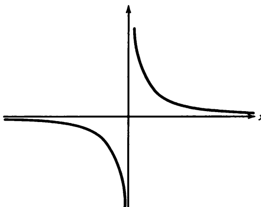
Figure 4.3.4 Graph of g(x) = 1/x ( x \neq 0 )
