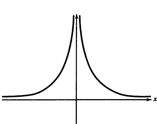
Figure 4.3.3 Graph of f(x) = 1/x^2 ( x \neq 0 )
