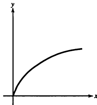
Figure 5.6.5 Graph of g(x) = x^{1/n} ( x \geq 0, n even).
