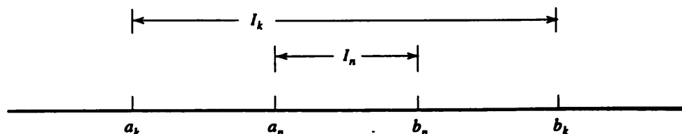
Figure 2.5.2 If k < n , then I_n \subseteq I_k
