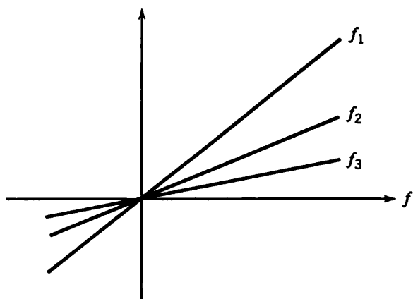
Figure 8.1.1 f_n(x) = x/n .
