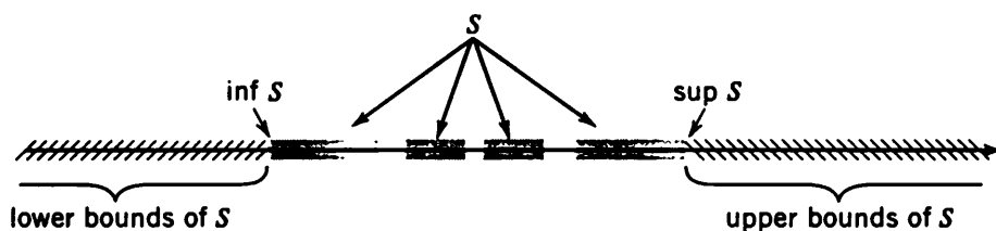
Figure 2.3.1 \inf S and \sup S
